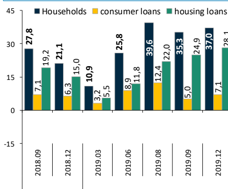
Cumulative changes (PLN bn)
